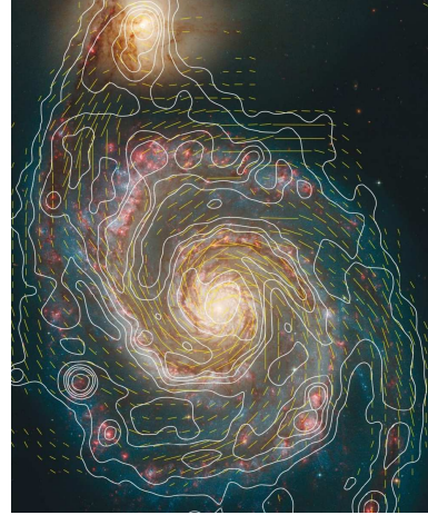
Figure 4: Total radio emission (contours) and B -vectors of M 51, combined from observations at 6 cm wavelength with the VLA and Effelsberg telescopes and smoothed to 15'' resolution, overlaid onto an optical image from the HST. Copyright: MPIfR Bonn and Hubble Heritage Team . Graphics: Sterne und Weltraum (from [28]).
