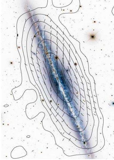
Figure 5: Total radio emission (84'' resolution) and B -vectors of the edge-on galaxy NGC 891, a galaxy similar to the Milky Way, observed at 8.4 MHz with the Effelsberg telescope. The background optical image is from the CFHT. Copyright: MPIfR Bonn and CFHT/Coelum (from [45]).
