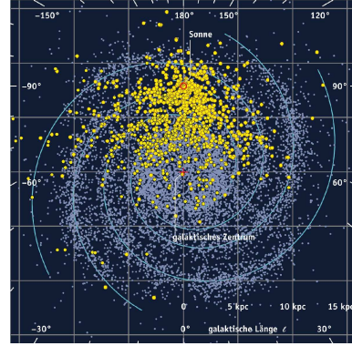
Figure 8: Simulation of about 20 000 pulsars (blue) in the Milky Way that will be detected with the SKA, compared to about 2000 pulsars known today (yellow). Graphics: Sterne und Weltraum (from Cordes, priv. comm).
