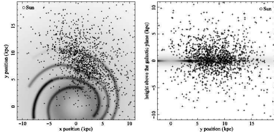
Figure 7: Simulation of the 1000+ pulsars that LOFAR is expected to find in a 60-day all-sky survey, shown in a Galactic plane projection (left) and an edge-on view of the Galactic plane (right) (from [70]).
