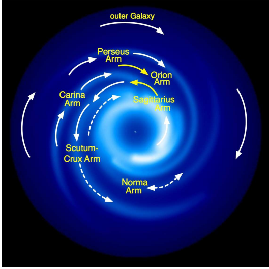
Figure 1: Sketch of the magnetic field in the Milky Way, as derived from Faraday rotation measures of pulsars and extragalactic sources. Generally accepted results are indicated by yellow vectors, while white vectors refer to results which need confirmation (from Brown, priv. comm.).
