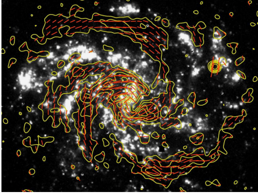
Figure 3: Polarized radio emission (contours) and B -vectors of NGC 6946, combined from observations at 6 cm wavelength with the VLA and Effelsberg 100m telescopes and smoothed to 15'' resolution (from [7]). The background image shows the H\alpha emission (from [26]). Copyright: MPIfR Bonn. Graphics: Sterne und Weltraum .
