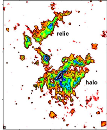
Figure 6: Total radio emission from the cluster A 2255, observed at 1.4 GHz with the VLA. The field size is about 20' x 25' (from [33]).
