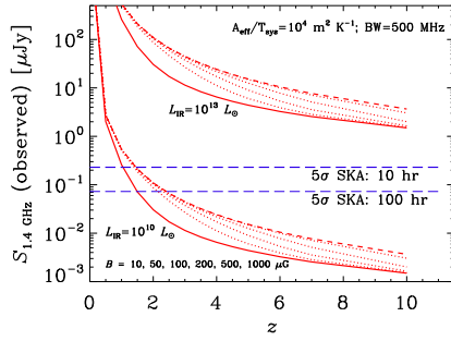
Figure 9: Synchrotron emission at 1.4 GHz as a function of redshift z and magnetic field strength B , and the 5\sigma detection limits for 10 h and 100 h integration time with the SKA (from [52]).
