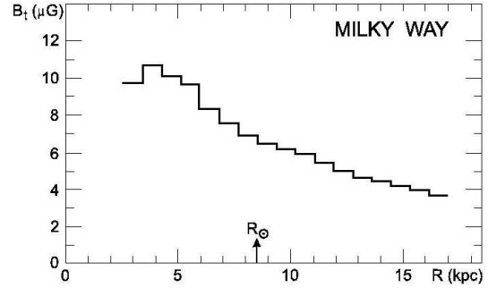
Figure 2: Strength of the total magnetic fields in the Milky Way, derived from the 408 MHz synchrotron emission, assuming equipartition between the energy densities of magnetic fields and cosmic rays (from Berkhuijsen, in [74]).
