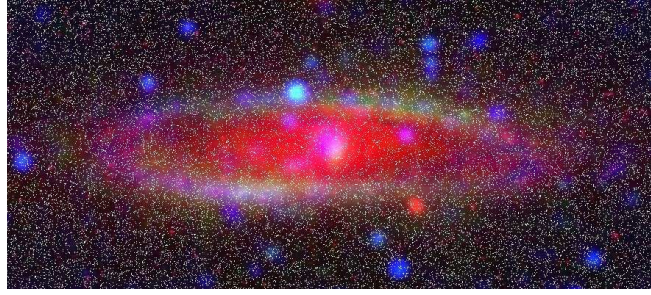
Figure 10: Simulation of RMs towards background sources (white points) in the region of M 31 observable with the SKA within 1 h. Optical emission from M 31 is shown in red, diffuse radio continuum intensity in blue and diffuse polarized intensity in green (from Gaensler, priv. comm.).
