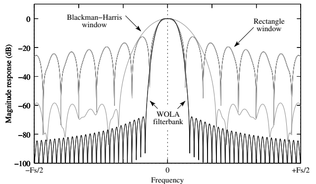
Figure 10. The frequency response of a single FFT bin is compared to an unweighted FFT (rectangle window), a Blackman-Harris window and to the WOLA method.
