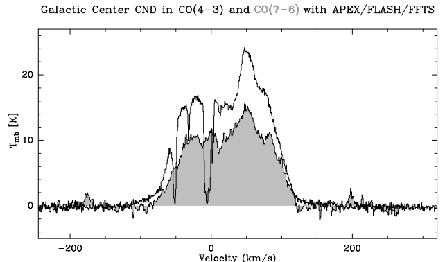
Figure 14. Spatially averaged CO spectra towards the innermost \pm 30 arcsec of the Galactic Center, observed with FLASH. The emission of CO(4-3) (top spectrum), observed with 1 GHz bandwidth, is superimposed on the CO(7-6) line (filled grey) observed with 1.6 GHz bandwidth - no baseline-fitting applied to these spectra. Clearly the prominent broad CO emission is visible, but also narrow absorption lines and high velocity emission features with velocities up to 200 km/s can be identified. These spectra clearly show the advantage of having a wide spectral coverage with high resolution, allowing for simultaneous observation of a broad emission spectrum and relatively narrow line-of-sight absorptions.
