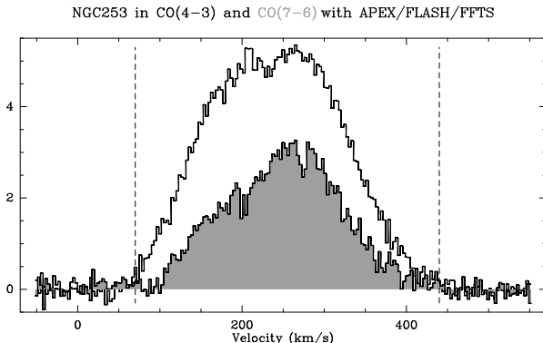
Figure 13. Spectra of warm carbon monoxide towards the nucleus of NGC 253, observed with the FLASH receiver at APEX. 23 The emission of CO(4-3) (at 461 GHz, top line), observed with 1 GHz bandwidth, is superimposed on the CO(7-6) line (806 GHz). The latter has been observed with an effective bandwidth of 1.8 GHz (composed of two 1 GHz bands, offset by 800 MHz). The dashed vertical lines indicate the bandwidth of 1 GHz for the CO(7-6) line. Clearly, the velocity width is barely sufficient to define the zero level (baseline), emphasizing the need for wide bandwidth spectrometers for extragalactic work at submm frequencies.
