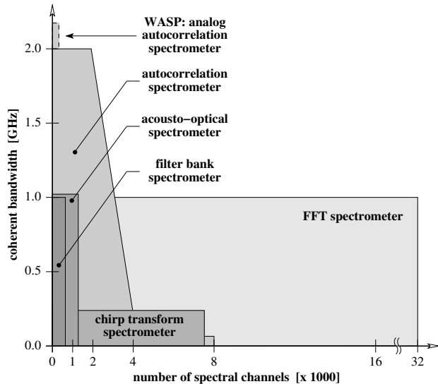
Figure 1. Comparison of different spectrometer types in terms of coherent bandwidth and spectral channel number applied in radio astronomy. Only FFT spectrometers provide both wide bandwidths and an impressive number of spectral channels, thus high frequency resolution.
