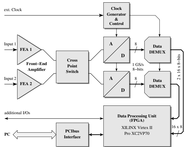
Figure 4. Block diagram of Acqiris' AC240 digitizer/analyser board, the main hardware of the APEX FFT spectrometer. By applying interleaved techniques, the two 1 GS/s 8-bits ADCs can be combined to one 2 GS/s converter. To feed the high data rate output of the ADCs (2 GBytes/s) to the FPGA, de-multiplexers (DEMUX) are used which split the two 8-bits data streams at 1 GHz to 2 \times 16 streams at 62.5 MHz, suitable for the FPGA.
