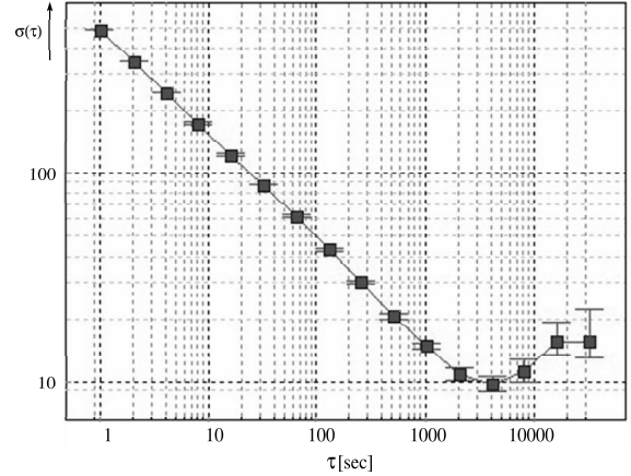
Figure 12. The remarkable stability of the APEX FFTS is illustrated in this Allan-Variance-Plot. The spectrum of a noise source (0-1 GHz) was integrated and processed in the FFTS. The spectroscopic variance between two 1 MHz broad channels, separated by 600 MHz within the band, was determined to be stable on a timescale of \sim 4000 s.
