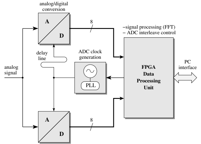
Figure 8. Functional diagram of two time-interleaved ADCs: Interleaving two ADCs is the process of using a second ADC with 180 degree phase-shift to fill data half way between the samples of the first ADC.
