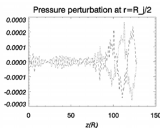
Figure 3. Axial cut of pressure perturbation at R_j/2 for the linear region of growth of the modes. We can identify three different structures: antisymmetric (helical) \lambda \sim 4 (all through the cut) and \lambda \sim 25 R_j (from 80 R_j ) modes and a symmetric (elliptic) \lambda \sim 50 R_j (up to 80 R_j ) mode. Dashed and dotted lines stand for symmetric points around the jet axis.
