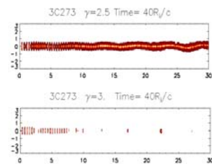
Figure 5. Surface plots for Lorentz factors 2.5 and 3.
