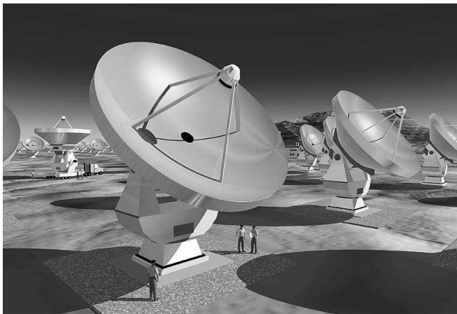
Figure 10: Artist's impression of ALMA.
