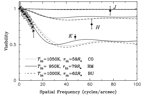
Fig. 2: The filled diamond represents the JHK -band visibilities observed with IOTA along P.A. \sim 170^\circ . The visibility obtained at near-maximum light in 1996 is represented by filled circles. Model predictions with different dust opacities are represented by 3 curves. RM: Rouleau & Martin (1991), CO: Colangeli et al. (1995), BU: Bussoletti et al. (1987)
