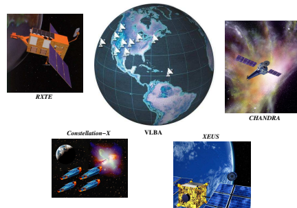
Present and future X-ray missions suitable for combined VLBI- and X-ray spectroscopic observations of radio-loud AGN.
